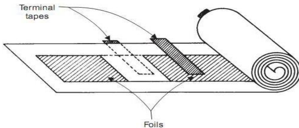
Fig. 1.20. Impregnated paper capacitor-terminal tape type
