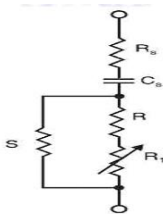
Fig. 6.12 Shunt arrangement for measurement of large capacitance
