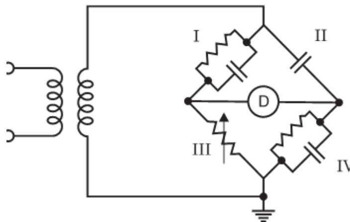
Fig. Basic high voltage schering bridge
