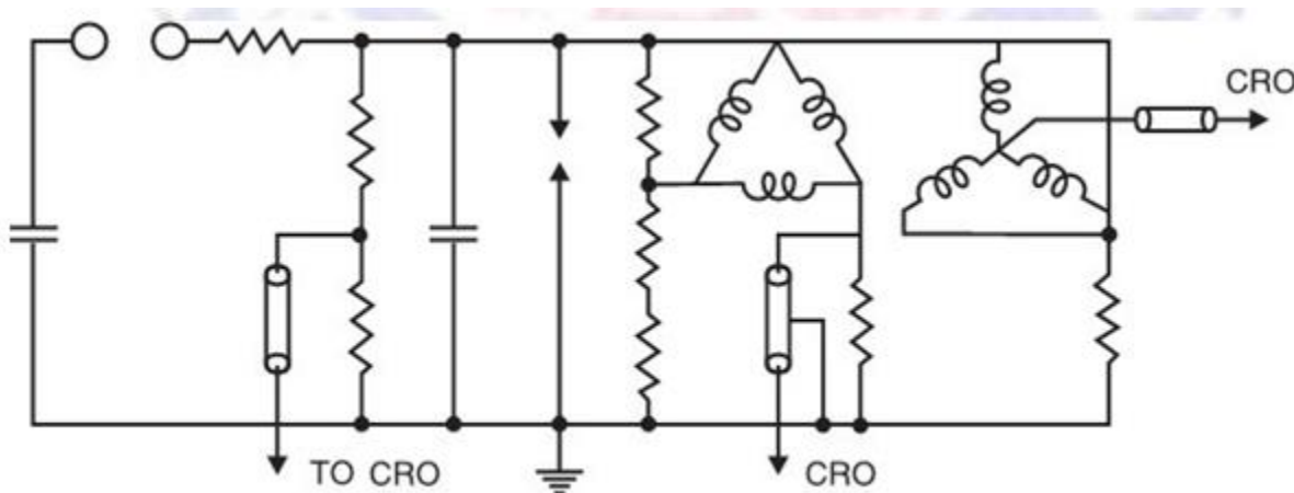
Fig. 5.3 Arrangement for impulse testing of transformer
